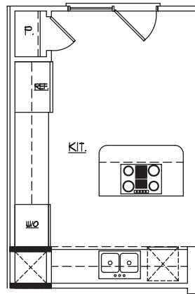
PART. FIRST FLOOR PLAN W/ OPT. GOURMET KITCHEN SCALE: 1/4"=1'-0"
